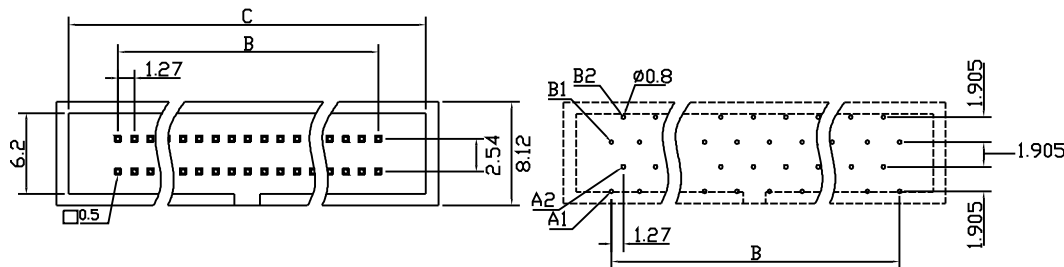
P.C. Board Layout Top View (26,34,50 Position)
